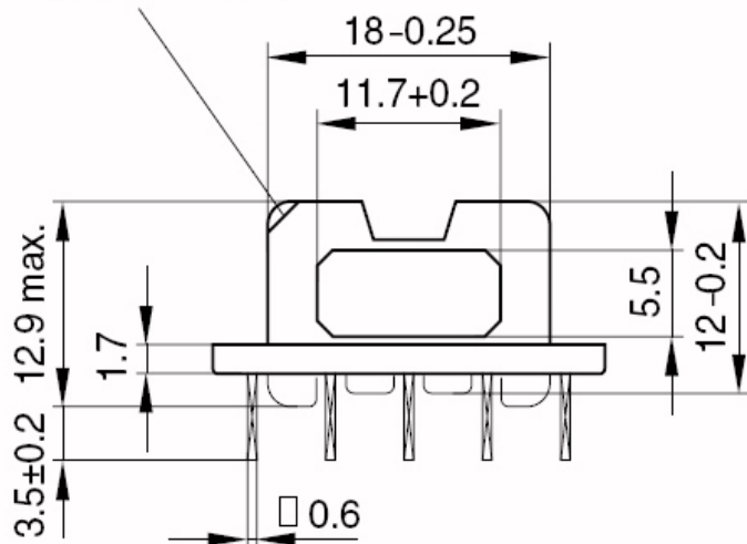
Pin 1 marking
