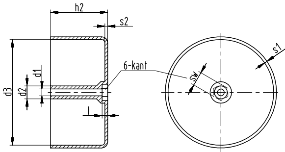
Sketch with main dimensions
