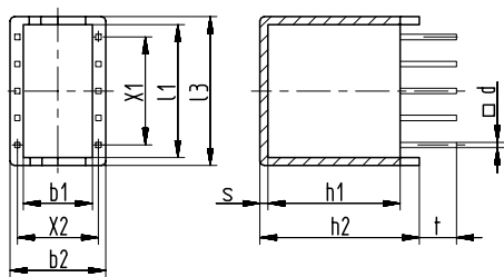
Sketch with main dimensions
